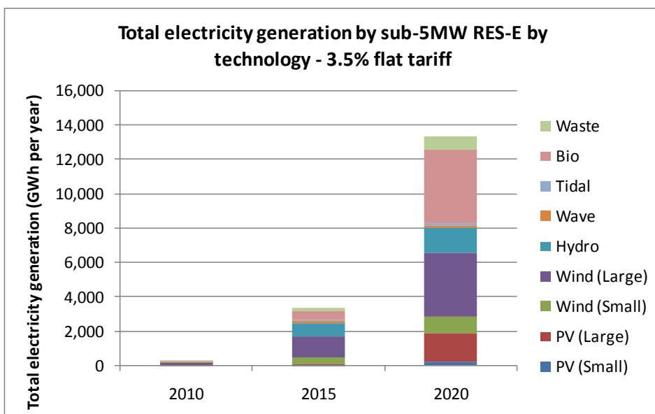
Figure 20 Electricity generation in 2020 - £270 flat tariff
